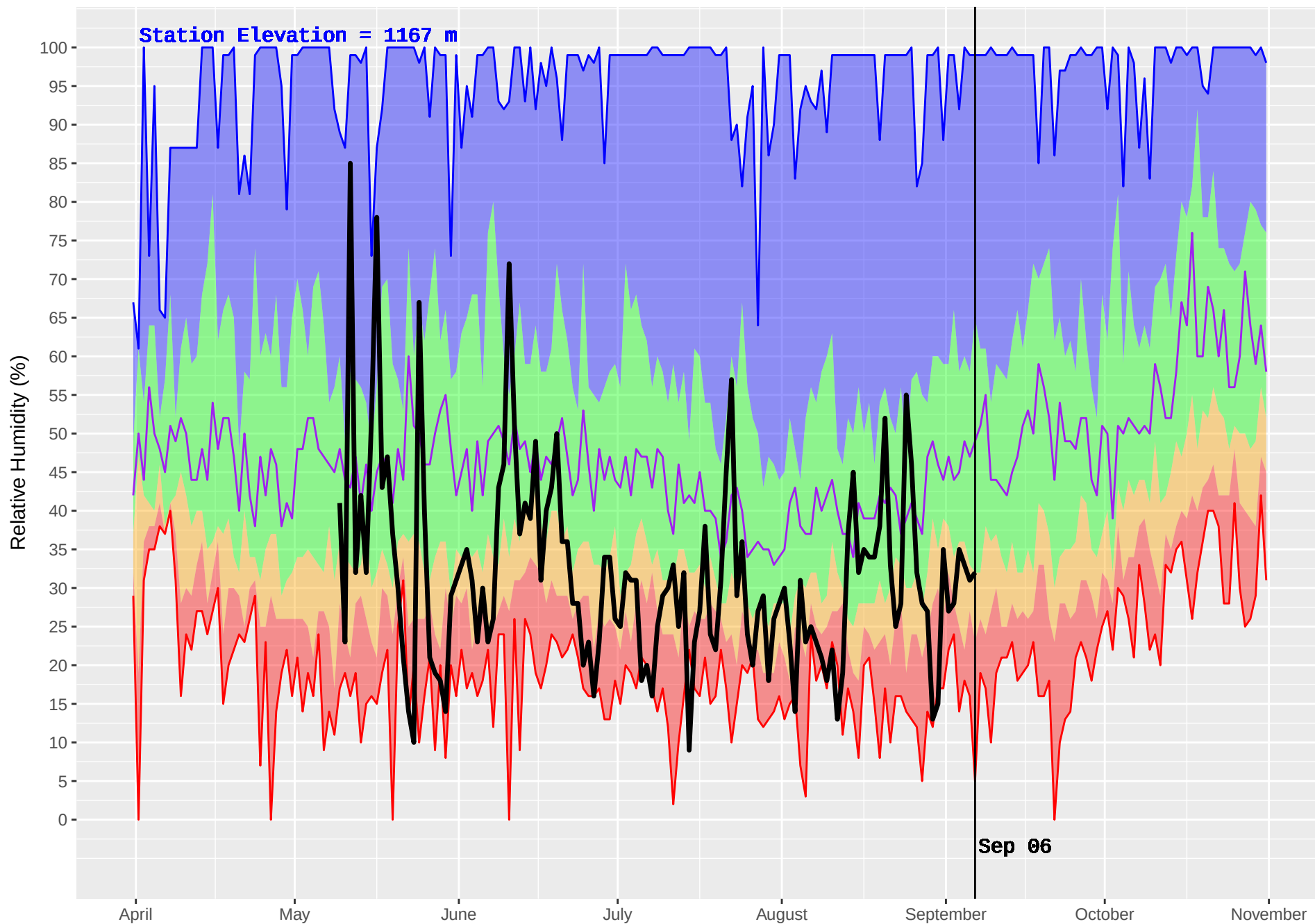
LEIGHTON LAKE (307) : Historical (1982–2016) and Current (2017) Noon Relative Humidity
