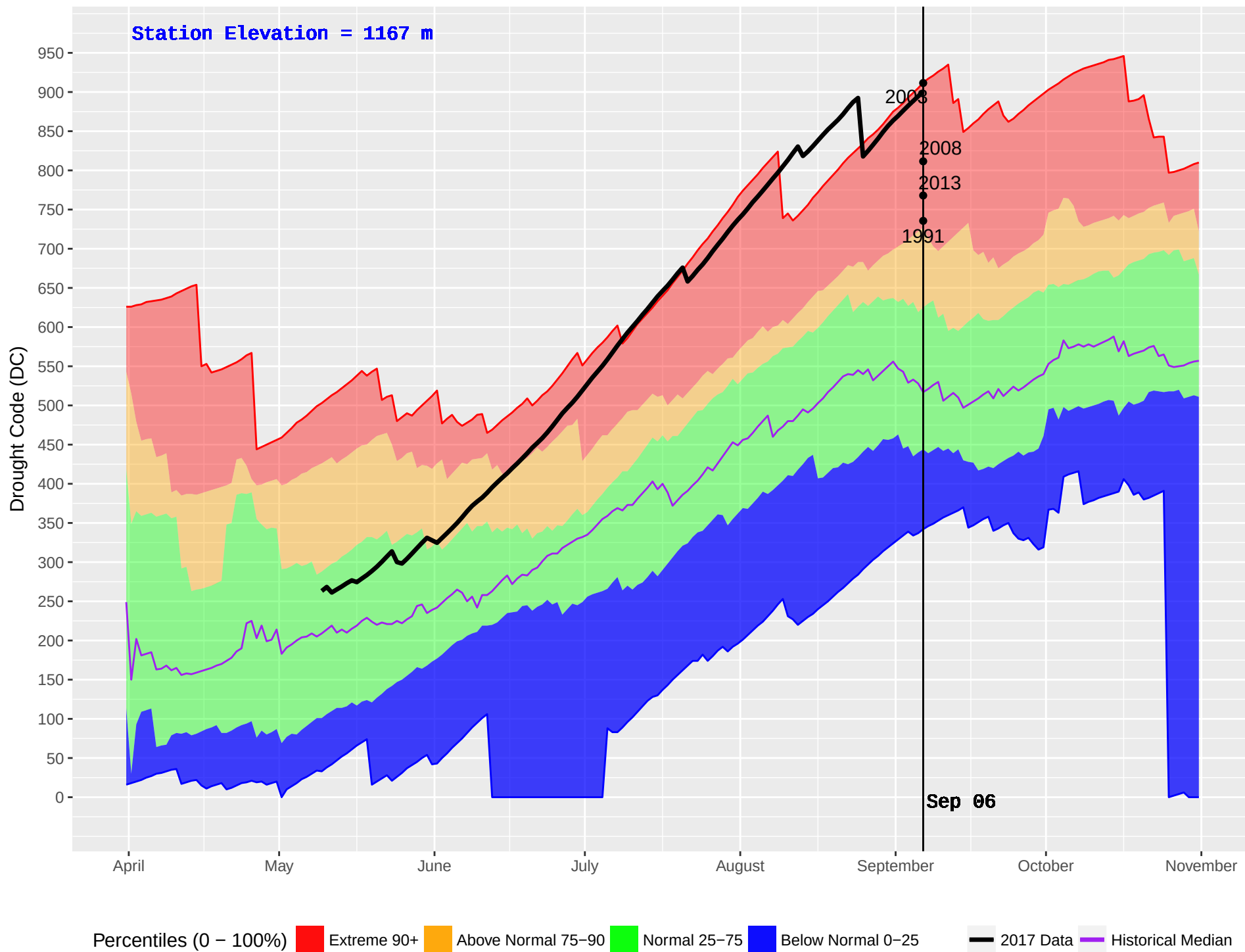
LEIGHTON LAKE (307) : Historical (1982–2016) and Current (2017) Noon Drought Code (DC)
