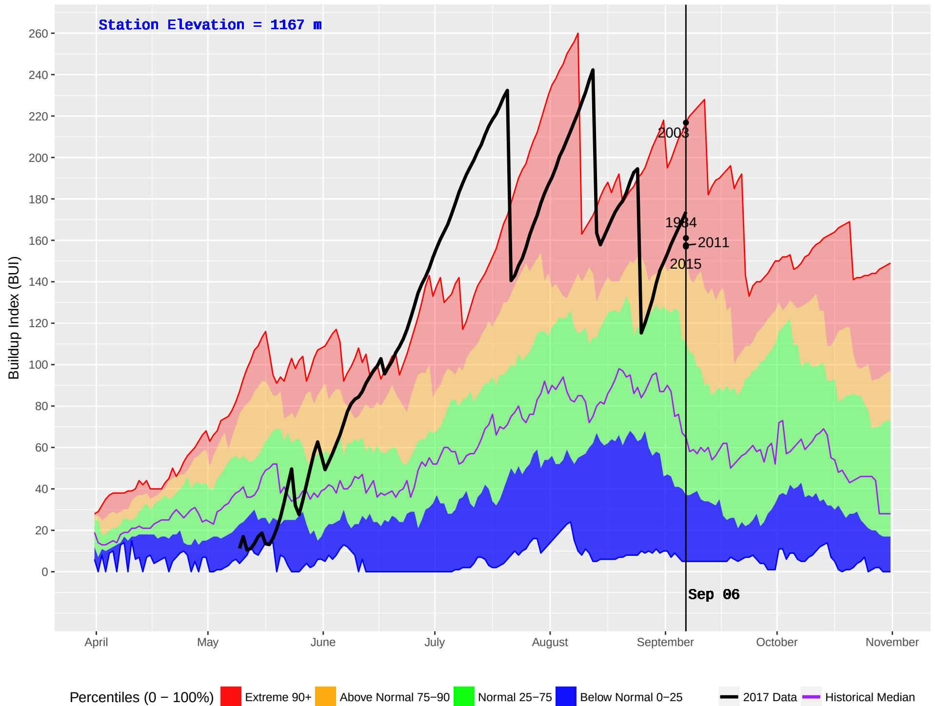
LEIGHTON LAKE (307) : Historical (1982–2016) and Current (2017) Noon Buildup Index (BUI)
