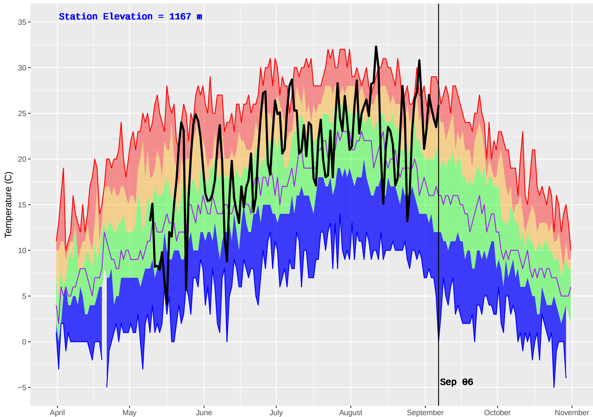
LEIGHTON LAKE (307) : Historical (1982–2016) and Current (2017) Noon Temperature
